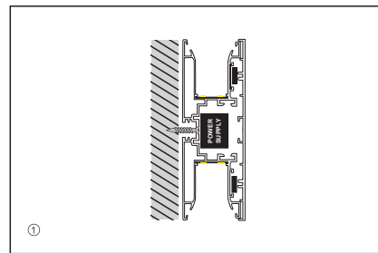
① Installing profiles to wall
