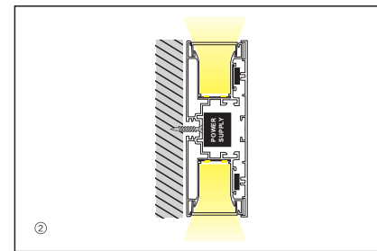
② Installation of driver, light source pc cover and end cap Complete Fixed
