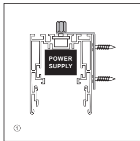
① Installing profiles to wall
