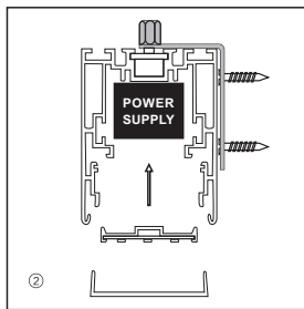
② Installation of driver, light source pc cover and end cap
